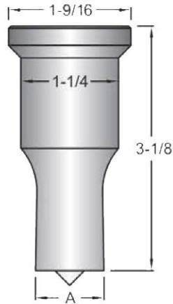
770 Punch
