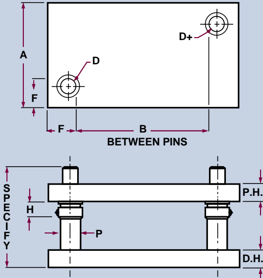
DIAGONAL PINS, TYPE D2
