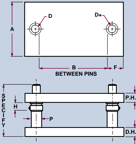
CENTER PINS, TYPE C2
